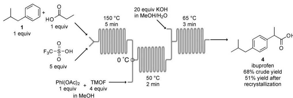
Figure 4. The three-step, continuous-flow synthesis of ibuprofen.
