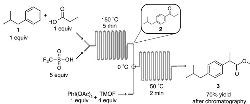
Figure 3. The two-step reaction sequence to methyl ester 3 .
